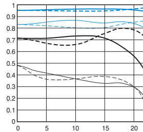
MTF Graph for EF 85mm f/1.2L II USM
